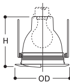
Height: 5" [127mm] Outside Diameter: 7-1/4" [184mm]
