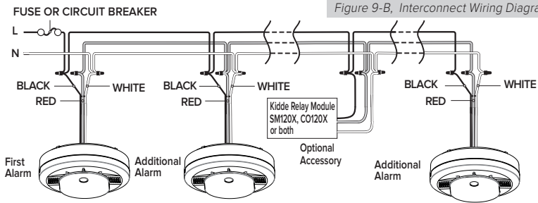
Figure 9-B, Interconnect Wiring Diagram
